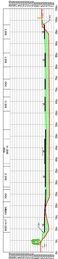
SECTION E-E 1:200
