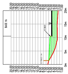
SECTION G-G 1:200
